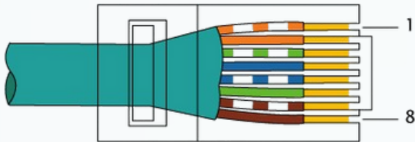
EIA/TIA-568B
